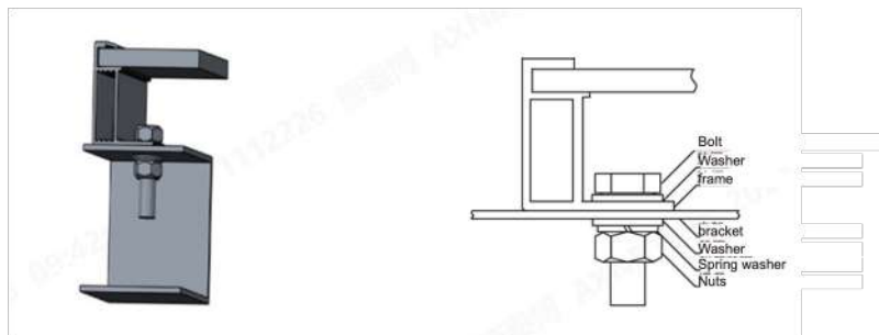
Module Mounting Holes
